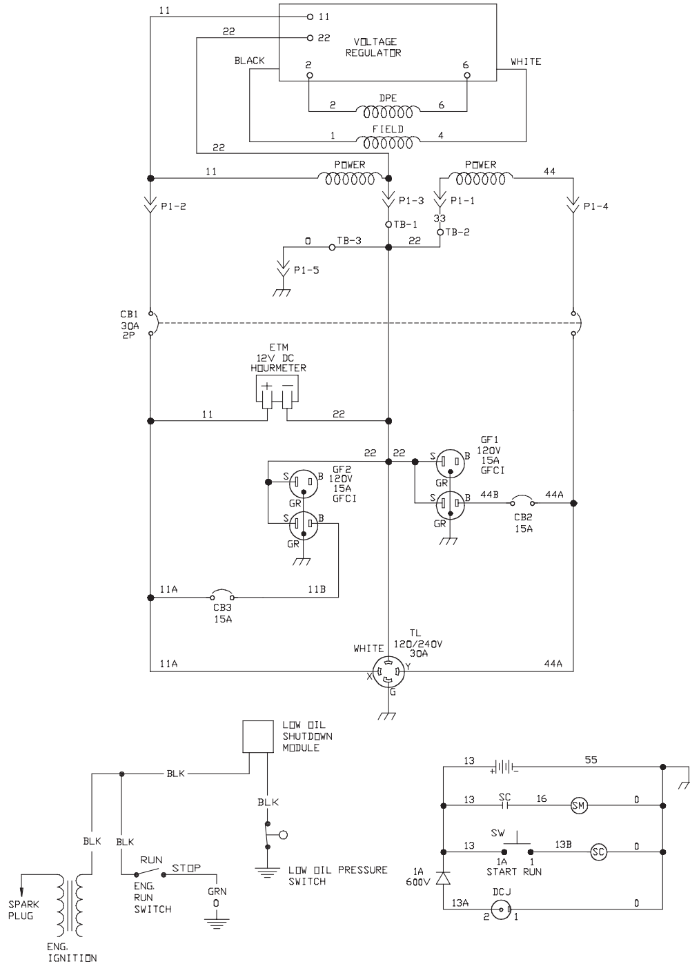
SCHEMATIC
